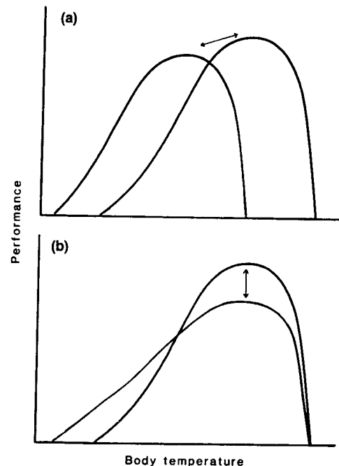
Fig. 3. (a) Performance curves predicted if 'hotter is better': the maximal absolute performance of a species increases directly with its optimal temperature. (b) Performance curves predicted if a 'jack-of-all-temperatures is a master of none': a trade-off exists between the maximum and the breadth of performance. After Ref. 16, with permission of the Society for the Study of Evolution.
